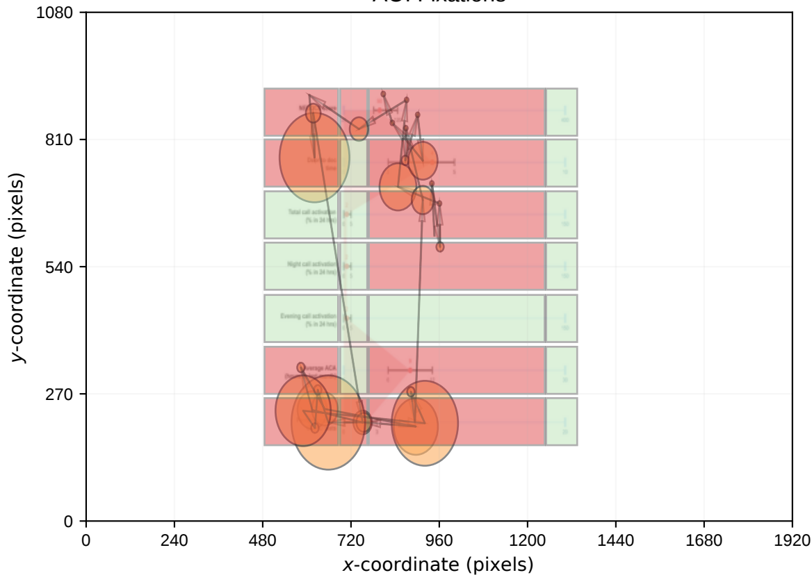
AOI Fixations
